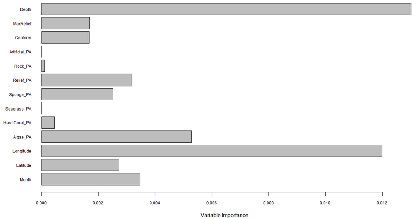
Fig. 2. Example of variable importance ranking before fitting the final CART habitat model for red snapper with the FWRI data.
