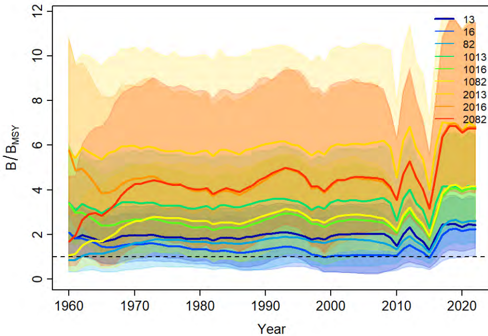
Figure 28: B/B msy estimates for Pink Shrimp across runs.
