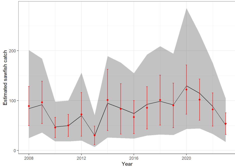
Bayesian model compared (line and shading of 95% C.I.) to ratio estimate (Red C.I. are 2 standard errors)
