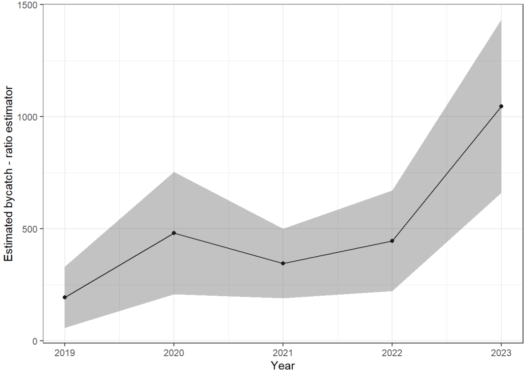
Design-based
