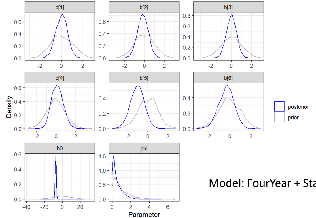
Prior and posterior densities of parameters for best Bayesian model
