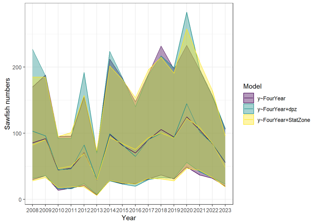
Model-based
