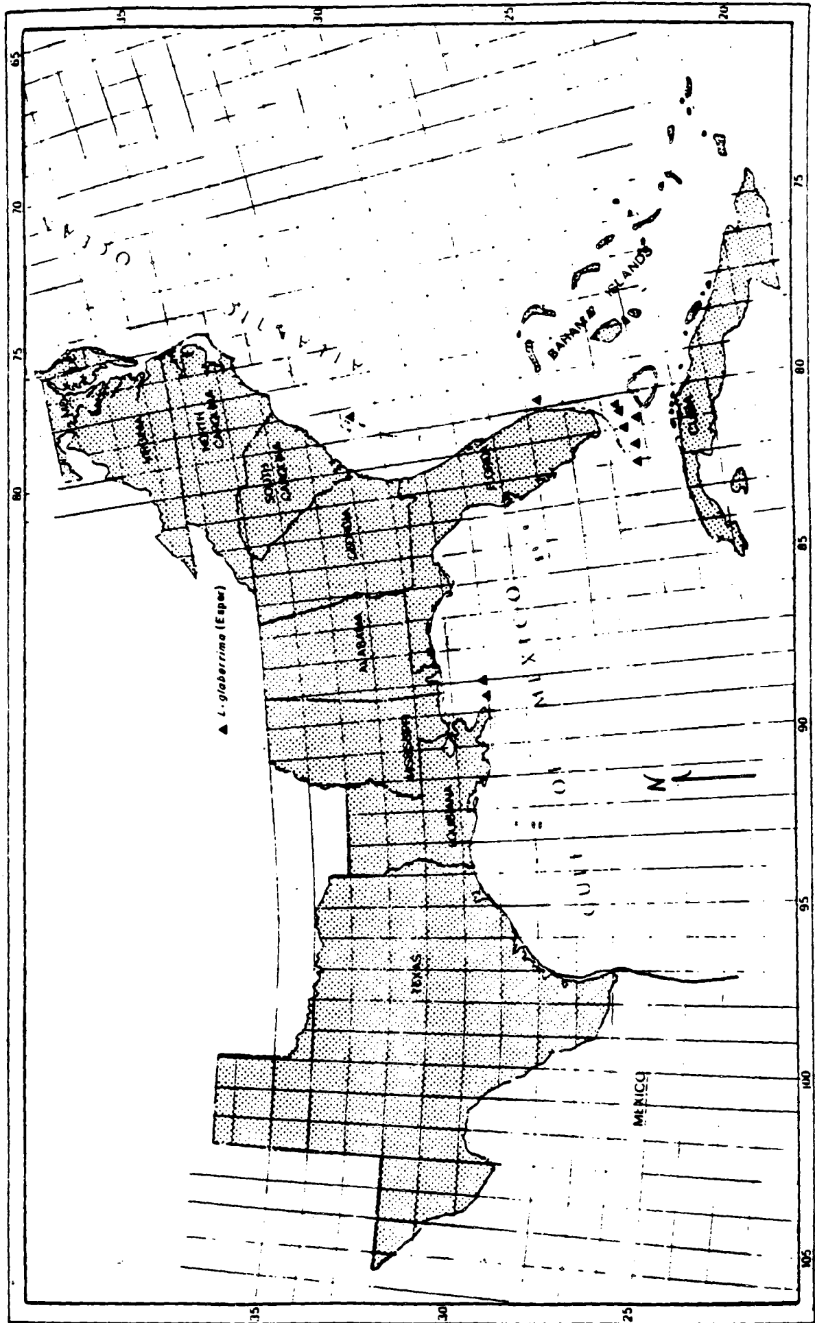
FIGURE D-5. Distribution of Leiopathes glaberrima in the vicinity of the management area.
