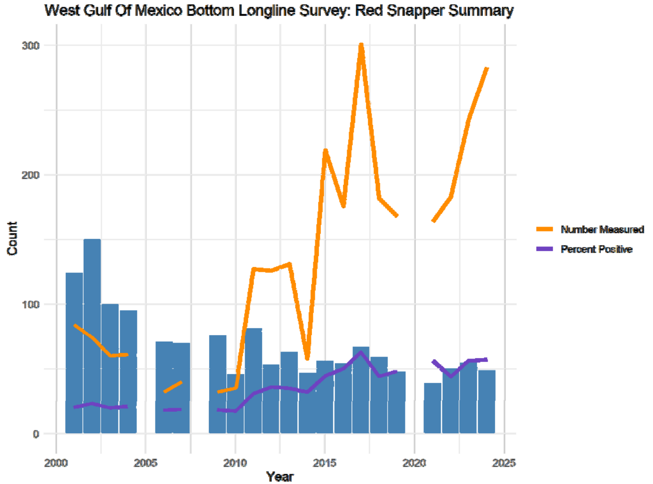
Figure 4. Summary of Western Gulf of Mexico NMFS Bottom Longline survey from 2001-2024. Blue bars represent the number of stations sampled annually, the orange line represents the number of red snapper measured each year and the purple line represents the percent of stations that caught at least one red snapper each year.
