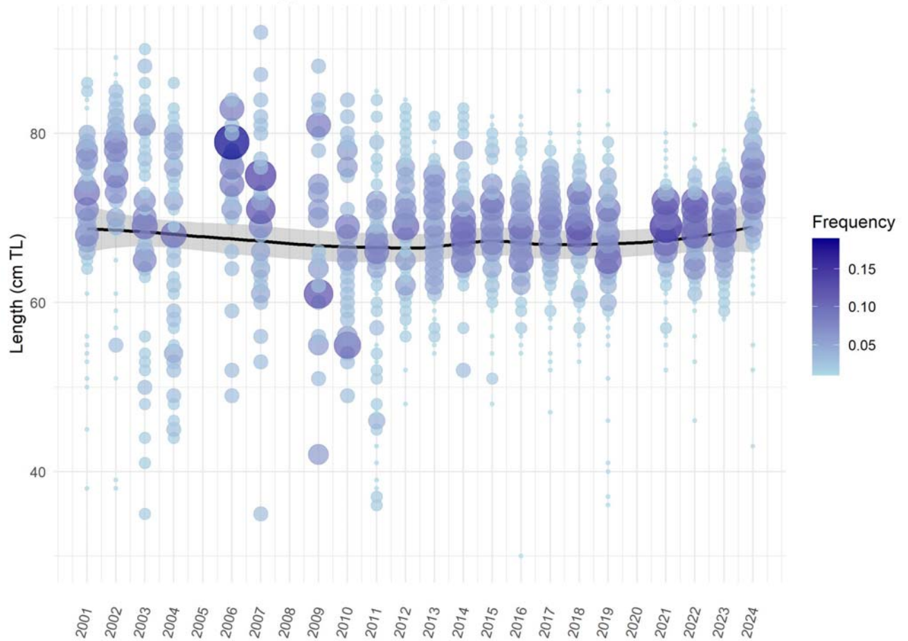
Figure 3. Summary of Western Gulf of Mexico red snapper length composition sampled in the NMFS Bottom Longline fishery independent survey from 2001-2024. Black line represents a long-term trend of size composition data.
