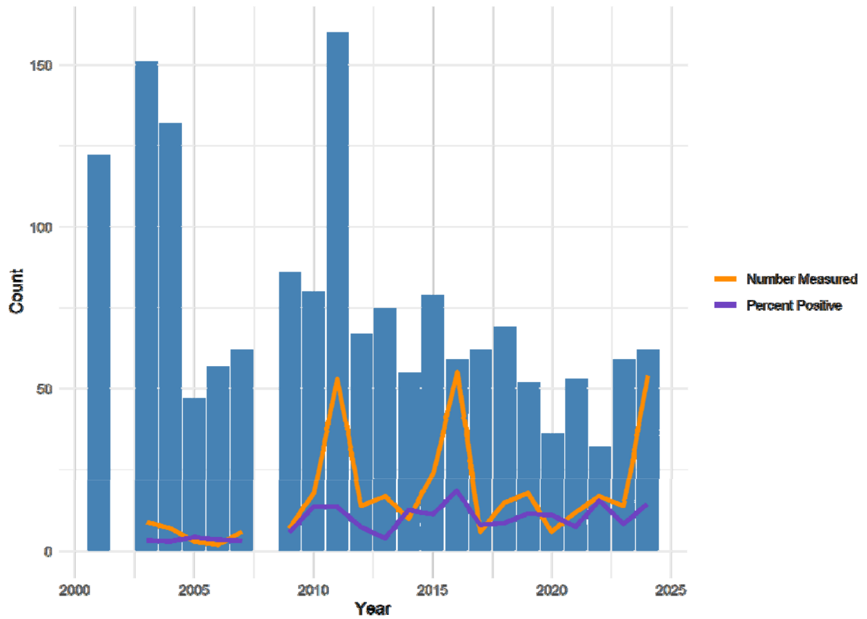
Figure 2. Summary of Eastern Gulf of Mexico NMFS Bottom Longline survey from 2001-2024. Blue bars represent the number of stations sampled annually, the orange line represents the number of red snapper measured each year and the purple line represents the percent of stations that caught at least one red snapper each year.
