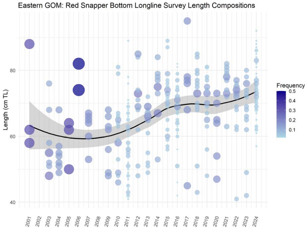
Figure 1. Summary of Eastern Gulf of Mexico red snapper length composition sampled in the NMFS Bottom Longline fishery independent survey from 2001-2024. Black line represents a long-term trend of size composition data.
